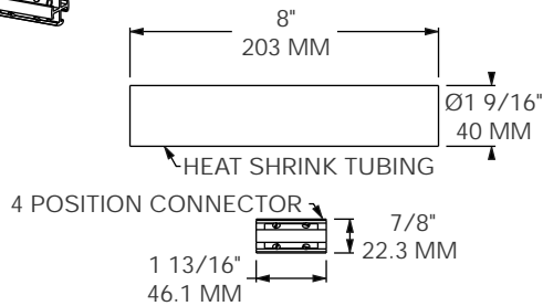
MODEL 2601-6273 SPLICE KIT, UF CABLE DIRECT BURIAL
