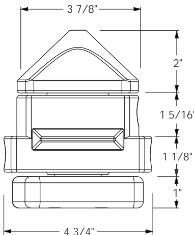
DETENTED LOCKED AND UNLOCKED POSITIONS
