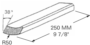
5203-10.71 x 32 - 38 5203-10.71 x 40 - 38 5203-10.94 x 50 - 38 END PIECE, CURVED R50 CUT AT 38° ANGLE
