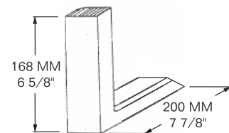
5203-10.71 x 32 - 90S 5203-10.71 x 40 - 90S 5203-10.94 x 50 - 90S 90° 'L' SHAPED CUT AT 45° ANGLE
