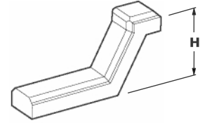
5203-10.71 x 32 - 3/150 5203-10.71 x 40 - 3/150 5203-10.94 x 50 - 3/150 THREE-WAY PAD, H = 150 MM
