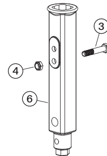
Extension Tube Assembly for 1101-3600-HA-9-NH-WL-KIT
