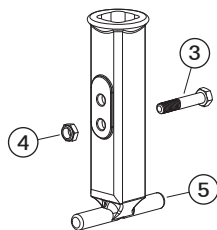
Handle Assembly for 1101-3600-HA-WL-KIT
