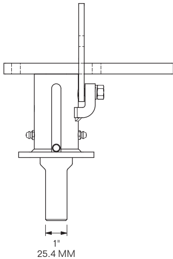
MODEL 1103-1624-R for Front Curbside
