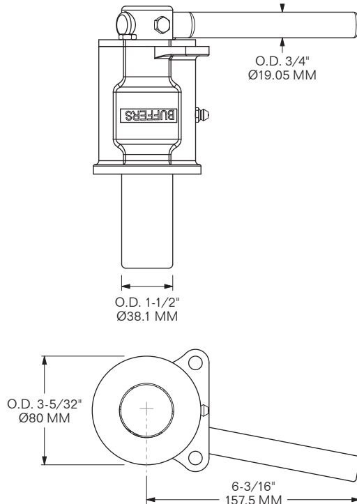
MODEL 1103-1212-L for Front Roadside
