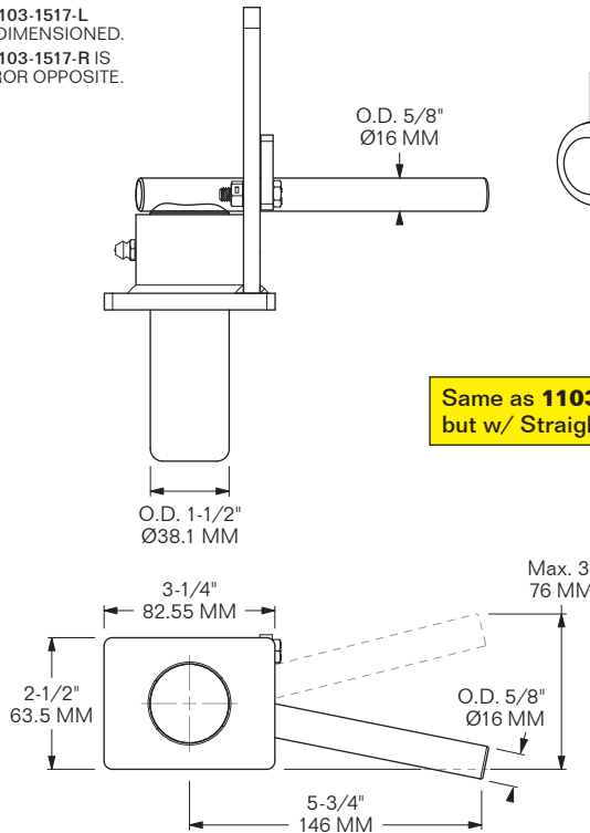
MODEL 1103-1517-L for Front Roadside
