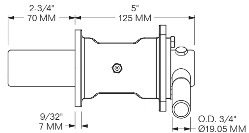
MODEL 1103-1212-R for Front Curbside
