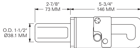
MODEL 1103-1617-R for Front Curbside
