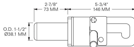
MODEL 1103-1517-R for Front Curbside
