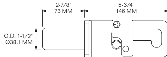
MODEL 1103-1417-R for Front Curbside
