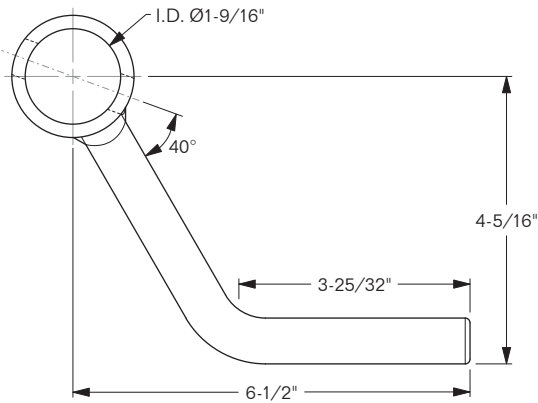
MODEL 1107-7351-R is shown dimensioned.
