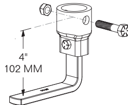
MODEL 1107-6942-102-KIT WEIGHT: 2.25 LBS / 1.02 Kg
