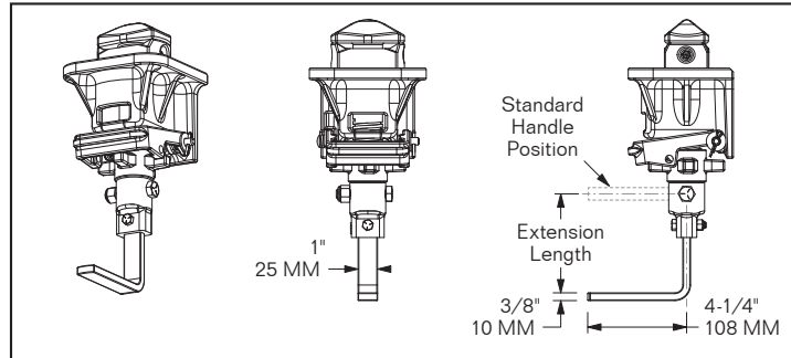
1107-7382 HANDLE EXTENSION BRACKET for Screwdown Twistlocks
