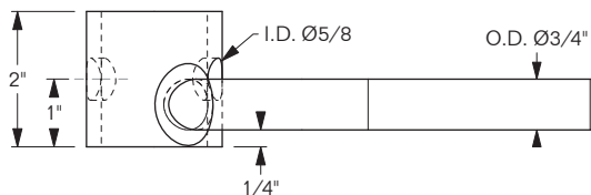
MODEL 1107-7351-R is shown dimensioned.
