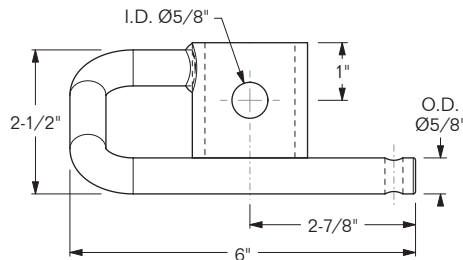
MODEL 1107-1728-R is shown dimensioned.
