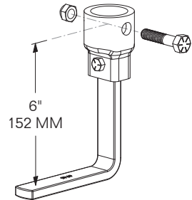
MODEL 1107-6942-152-KIT WEIGHT: 2.42 LBS / 1.1 Kg
