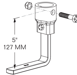
MODEL 1107-6942-127-KIT WEIGHT: 2.32 LBS / 1.05 Kg
