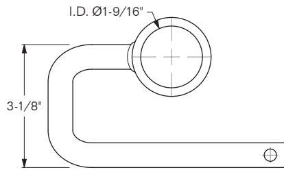
MODEL 1107-1728-R is shown dimensioned.
