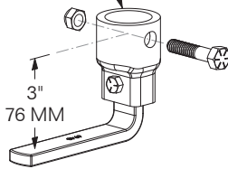
MODEL 1107-6942-76-KIT WEIGHT: 2.18 LBS / 0.99 Kg
