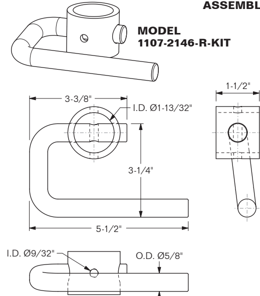
TWISTLOCK HANDLE ASSEMBLIES
