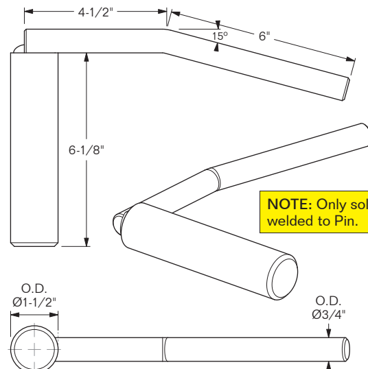
MODEL 1106-1759 PINLOCK PIN/HANDLE
