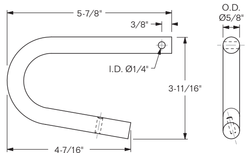
MODEL 1269-R HANDLE
