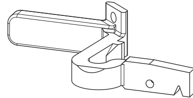
MODEL 1107-1375-L Rear Roadside / Front Curbside
