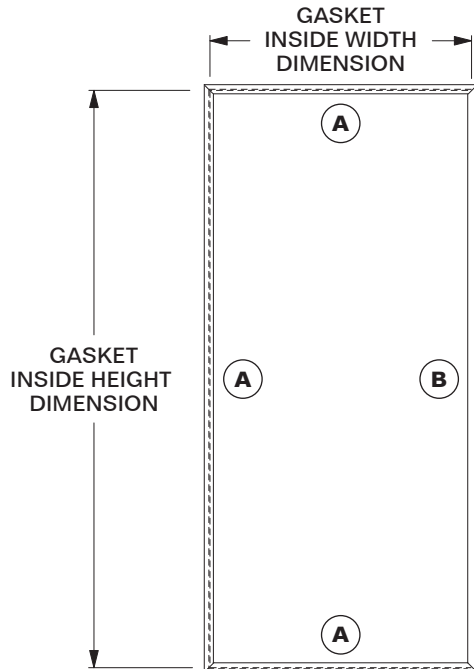
MODEL 1404-6830-L (8' 6") MODEL 1404-6831-L (9' 6") DOOR GASKET, INNER, LEFT
