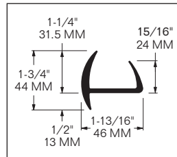
PROFILE A
