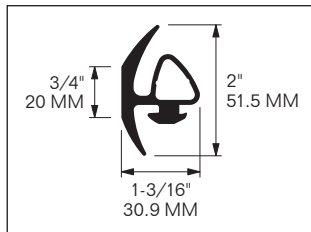
PROFILE A
