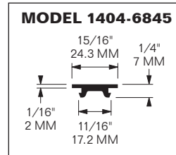
PROFILE B
