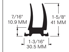
PROFILE A
