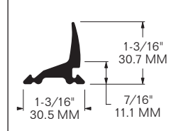
PROFILE B
