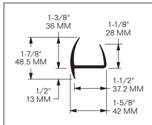
PROFILE A
