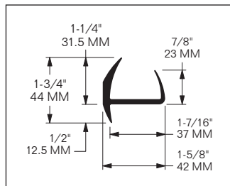
PROFILE A
