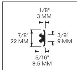
PROFILE B
