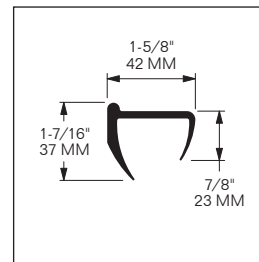
PROFILE C
