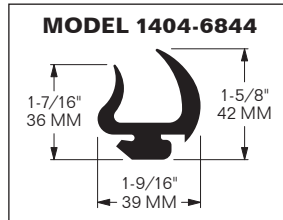
PROFILE A
