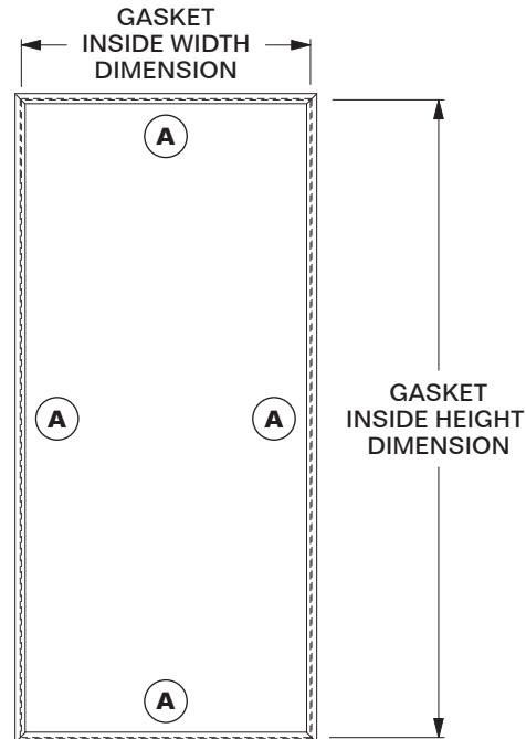
MODEL 1404-6830-R (8' 6") MODEL 1404-6831-R (9' 6") DOOR GASKET, INNER, RIGHT
