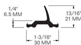
MODEL 1404-6247-B
