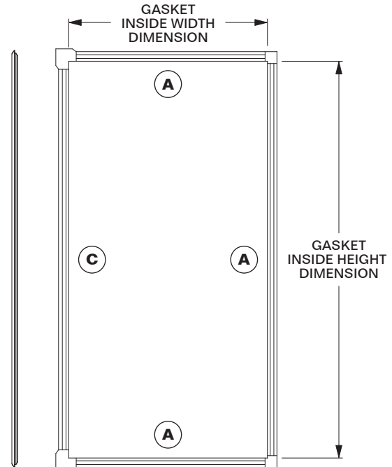
MODEL 1404-8954-R (8'6") MODEL 1404-8955-R (9'6") DOOR GASKET, Combo Design Inner & Outer, Right
