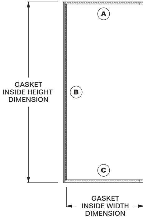
MODEL 1404-6935 3-SIDED OUTER DOOR GASKET
