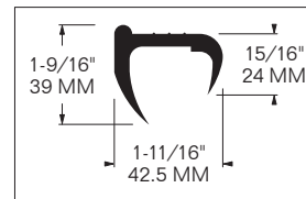
PROFILE B
