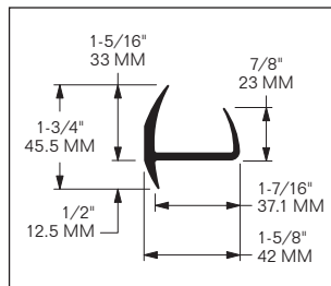
PROFILE B
