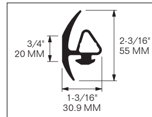
PROFILE C
