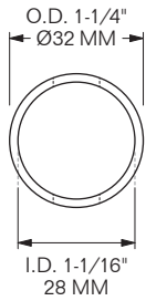
END TUBE 1-1/4" O.D. x 14 GA. TUBE w/ 7/16" x 3/4" SLOT
