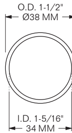
CENTER TUBE 1-1/2" O.D. x 14 GA.
